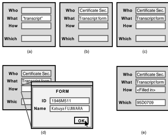
Figure 2. An example of operations of the MOON system at home.
