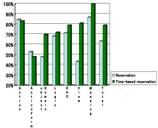
Fig.8. Reusability comparison
